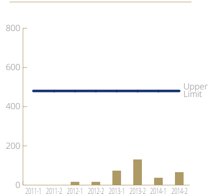
SO 2 LEVEL FROM BOILER (mg/L)
