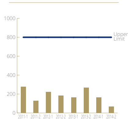
NO 2 LEVEL FROM BOILER (mg/L)
